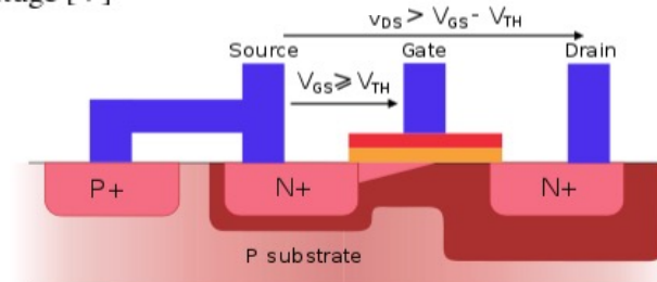
Saturation mode
